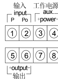
单相电压变送器 Single phase Voltage Transducer
