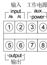
单相电流变送器 Single phase Current Transducer
